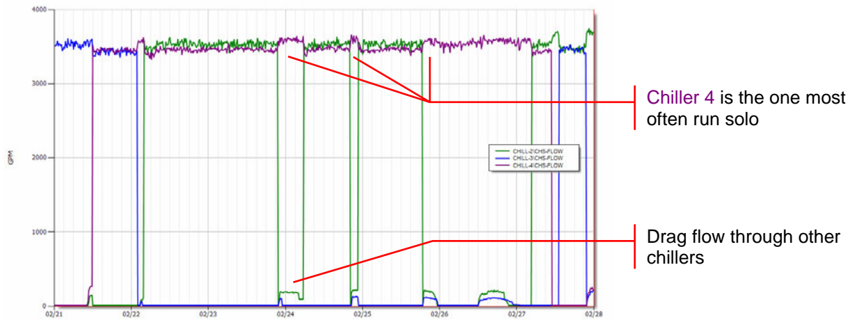
Figure H: Chiller Flows
